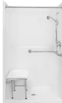
MP4836BF L/R 48" W x 36" D x 78" H ADA Barrier Free Shower w/Seat, L Grab Bar & Standard Shower Faucet Note: Curtain Rod and Handheld shower pictured above are optional upgrades.
